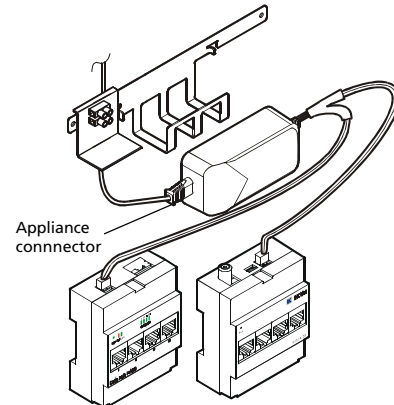
Figure 1: Power Supply for Data Hub and aerial module in external distribution board
