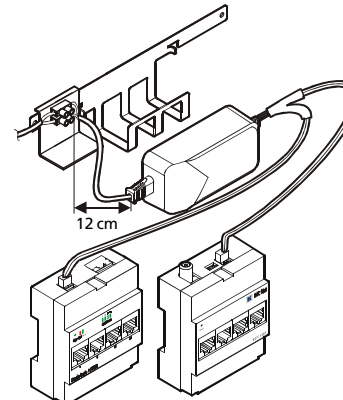
Figure 3: Installing power supply by use of mounting sleeve
