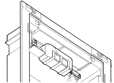
Figure 4: Power supply mounted in flush-mounted distribution board
