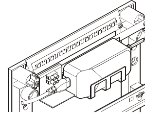
Figure 2: Power supply mounted in external distribution board
